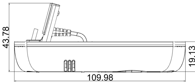
Left view
