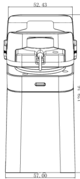
Back view
